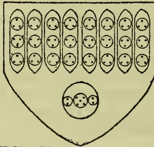
Gallium
